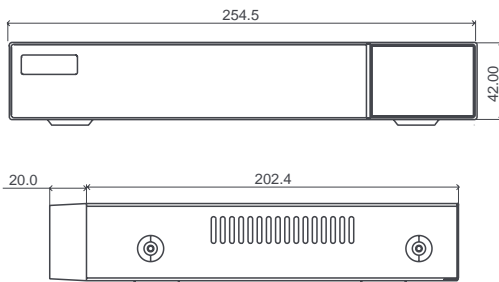
EWS-2104TS-HP
